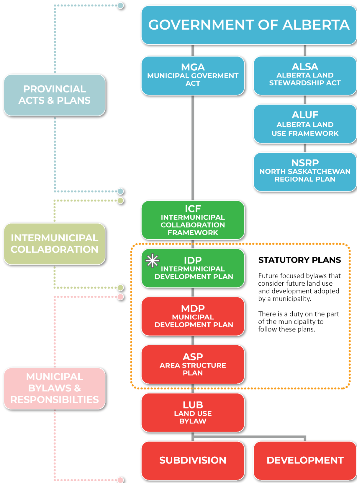
Figure 1: Planning Hierarchy
